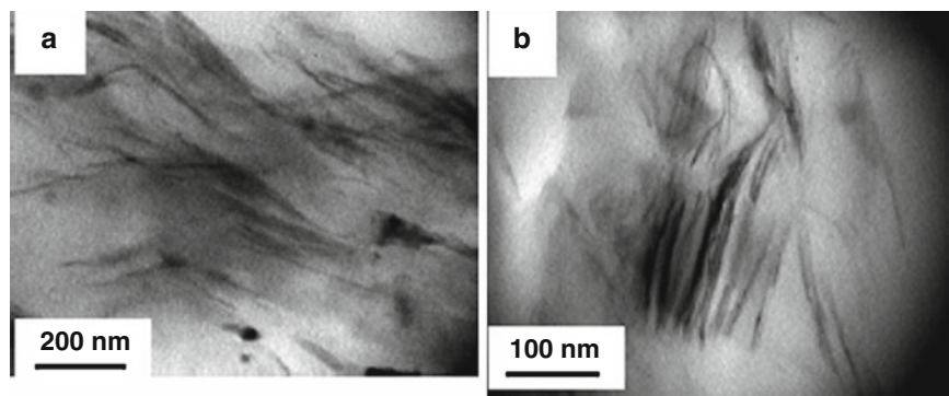
Fig. 20 TEM images of (a) (SIOHS-16)/Cloisite 15A ® nanocomposite and (b) (SIOHS-16)/Cloisite 30B ® nanocomposite, in which the dark areas represent the clay and the gray/white areas represent the polymer matrix. (Reprinted from Choi et al. [5]. Copyright 2004, with permission from the American Chemical Society)
