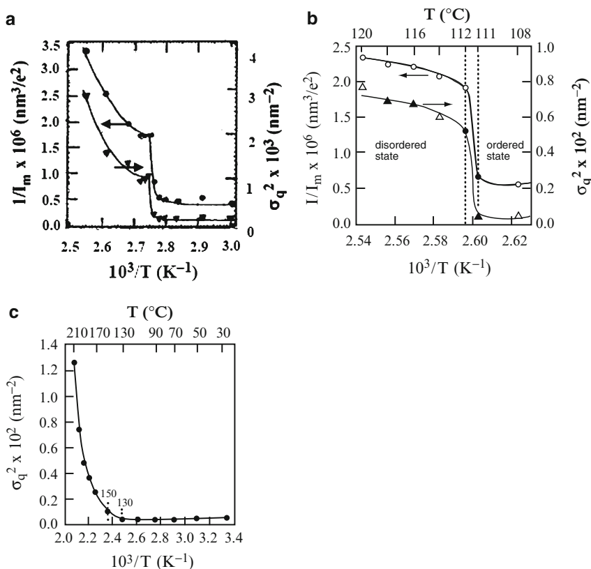
Fig. 17 Plots of 1/I_m vs 1/T and \sigma_q^2 vs 1/T for three SI diblock copolymers having different block length ratios. (a) SI-Z ( M_w = 1.93 \times 10^4 ; w_{PS} = 0.336 ; f_{PS} = 0.30 ). (b) SI-X ( M_w = 1.79 \times 10^4 ; w_{PS} = 0.50 ; f_{PS} = 0.46 ). (c) SI-L ( M_w = 4.10 \times 10^4 ; w_{PS} = 0.833 ; f_{PS} = 0.81 ). (Reprinted from Ogawa et al. [94]. Copyright © 1996, with permission from the American Chemical Society)
