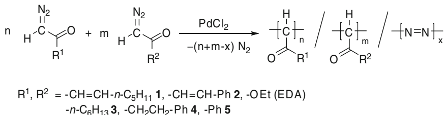
Scheme 22 \text{PdCl}_2 -mediated copolymerization of various diazocarbonyl compounds
