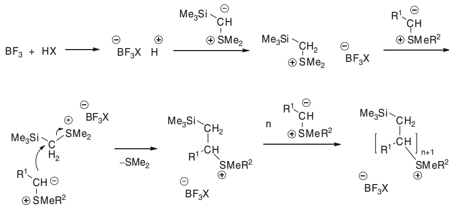
Scheme 58 Cationic mechanism for polymerization of sulfonium ylide
