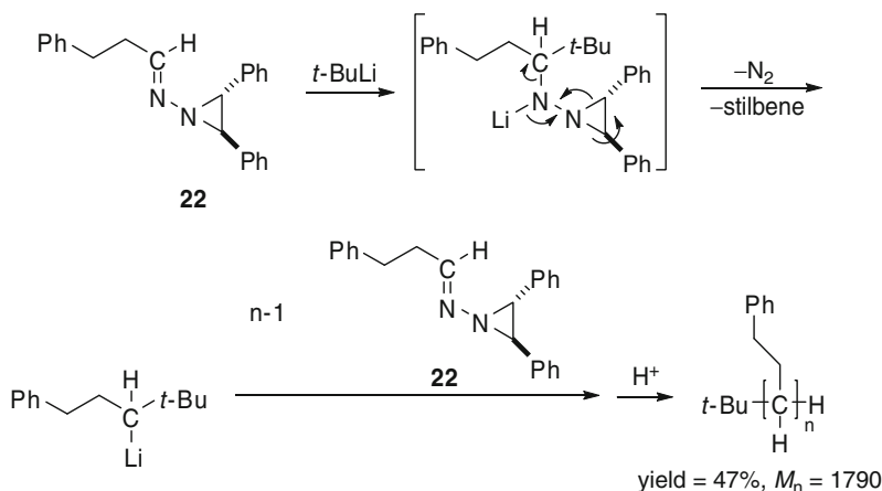
Scheme 59 Anionic polymerization of hydrocinnamaldehyde trans -1-amino-2,3-diphenylaziridine hydrazone 22
