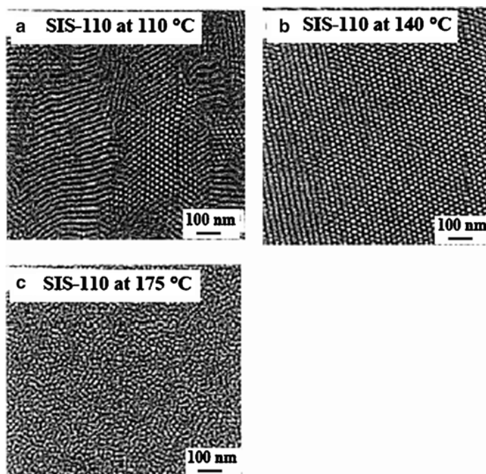
Fig. 25 TEM images of the highly asymmetric SIS-110, which had been annealed at 110°C for 3 days and then annealed further at: (a) 110°C for 1 h followed by a rapid quench in ice water; (b) 140°C for 1 h followed by a rapid quench in ice water; (c) 175°C for 1 h followed by a rapid quench in ice water. (Reprinted from Choi et al. [126]. Copyright © 2003, with permission from the American Chemical Society)
