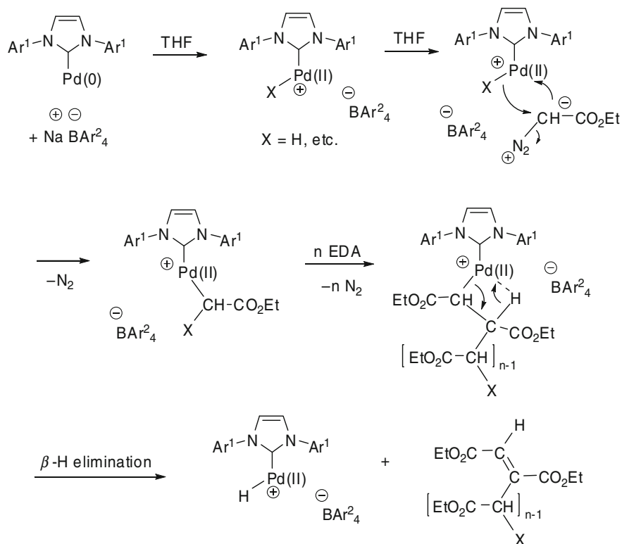
Scheme 17 Mechanism for (NHC)Pd/borate-initiated polymerization of ethyl diazoacetate
