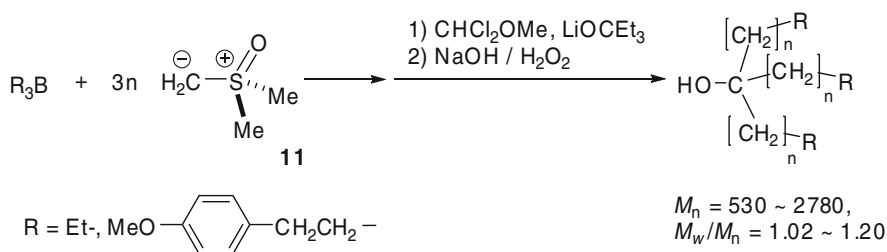
Scheme 50 Synthesis of three armed star polymethylene by R_3B -initiated polymerization of 11
