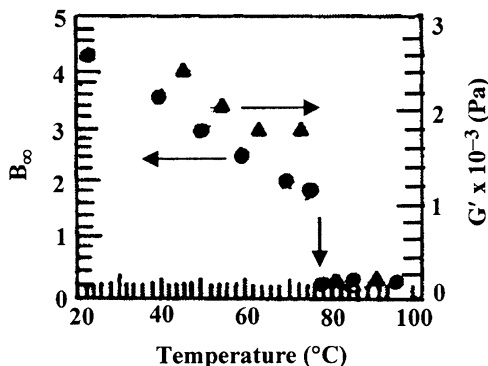
Fig. 21 Variation of birefringence ( B_{\infty} ) (●) and G' (▲) at \omega = 10 \text{ rad s}^{-1} with temperature for a 50.8/49.2 (w/w) SI diblock copolymer/bis(2-ethylhexyl)phthalate solution. (Reprinted from Balsara et al. [129]. Copyright © 1992, with permission from the American Chemical Society)
