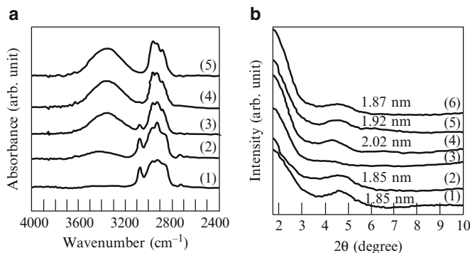
Fig. 3 (a) FTIR spectra for (1) PI, (2) PIOH-30, (3) PIOH-50, (4) PIOH-75, and (5) PIOH-100. (b) XRD patterns for (1) Cloisite 30B ® , (2) PI/Cloisite 30B ® nanocomposite, (3) (PIOH-30)/Cloisite 30B ® nanocomposite, (4) (PIOH-50)/Cloisite 30B ® nanocomposite, (5) (PIOH-75)/Cloisite 30B ® nanocomposite, and (6) (PIOH-100)/Cloisite 30B ® nanocomposite (Reprinted from Lee and Han [31]. Copyright 2003, with permission from the American Chemical Society)
