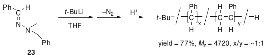
Scheme 60 Anionic polymerization of benzaldehyde 1-amino-2-phenylaziridine hydrazone 23 in THF
