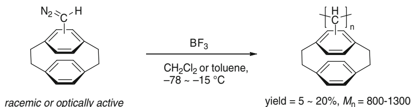
Scheme 5 \text{BF}_3 -mediated polymerization of paracyclophane-substituted diazomethane
