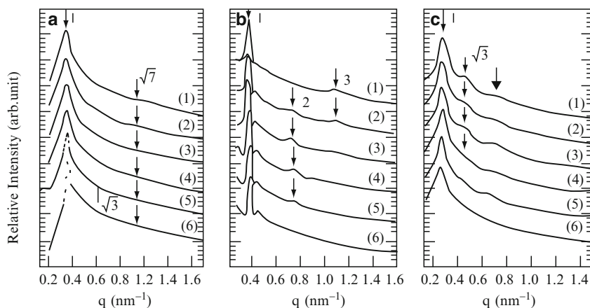
Fig. 16 SAXS profiles of three SI diblock copolymers having different block length ratios. (a) SI-Z ( M_w = 1.93 \times 10^4 ; w_{PS} = 0.336 ; f_{PS} = 0.30 ) at various temperatures ( ^{\circ}\text{C} ): (1) 30, (2) 50, (3) 60, (4) 70, (5) 80, and (6) 90. (b) SI-X ( M_w = 1.79 \times 10^4 ; w_{PS} = 0.50 ; f_{PS} = 0.46 ) at various temperatures ( ^{\circ}\text{C} ): (1) 25, (2) 50, (3) 70, (4) 90, (5) 100, and (6) 110. (c) SI-L ( M_w = 4.10 \times 10^4 ; w_{PS} = 0.833 ; f_{PS} = 0.81 ) at various temperatures ( ^{\circ}\text{C} ): (1) 26, (2) 50, (3) 70, (4) 90, (5) 110, and (6) 130. (Reprinted from Ogawa et al. [94]. Copyright © 1996, with permission from the American Chemical Society)
